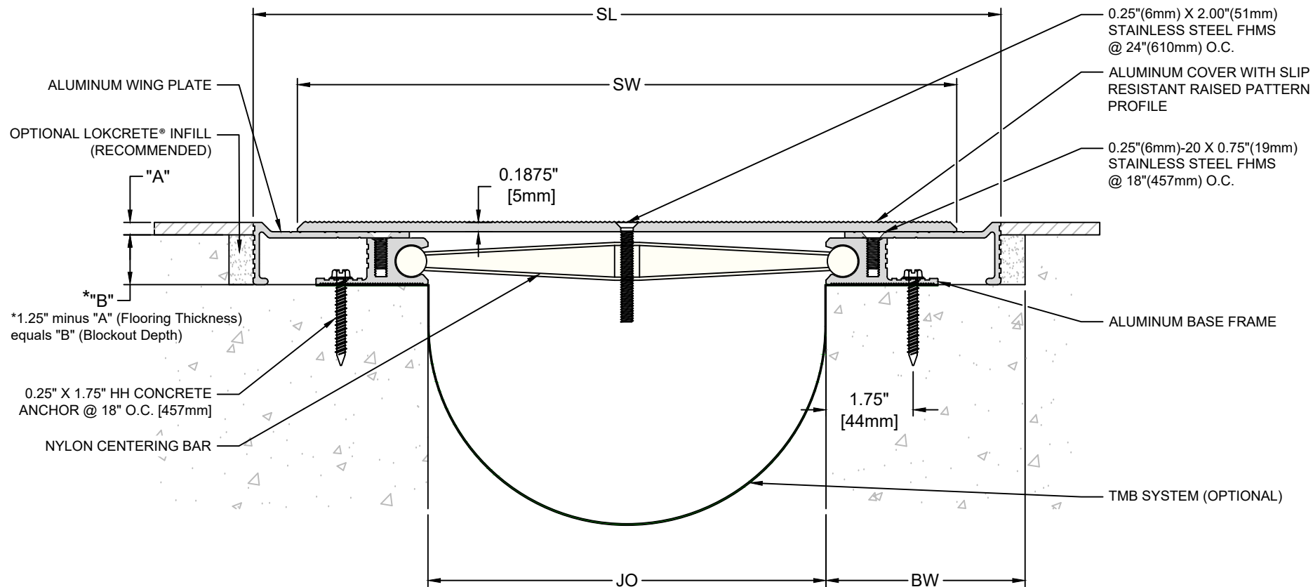
TFC Series Expansion Joint Sizes 200 Through 800 (Floor-to-Floor)
