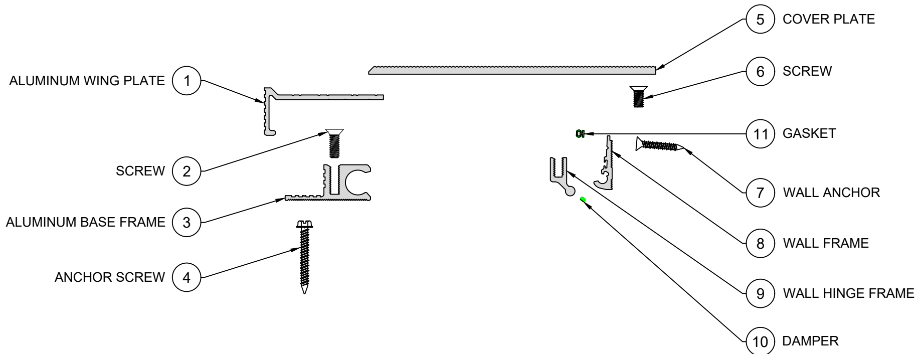
EXPLODED VIEW ▲
