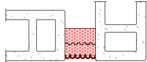
CMU BLOCK
