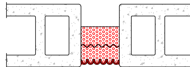
CMU BLOCK
