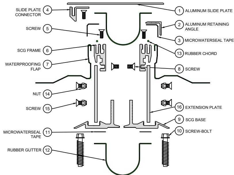
EXPLODED VIEW ▲
