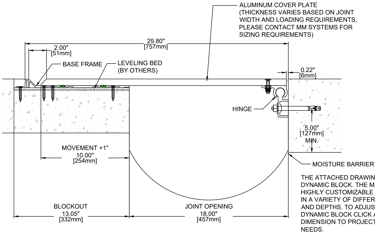
MJR Series Expansion Joint (Slab-to-Slab)
