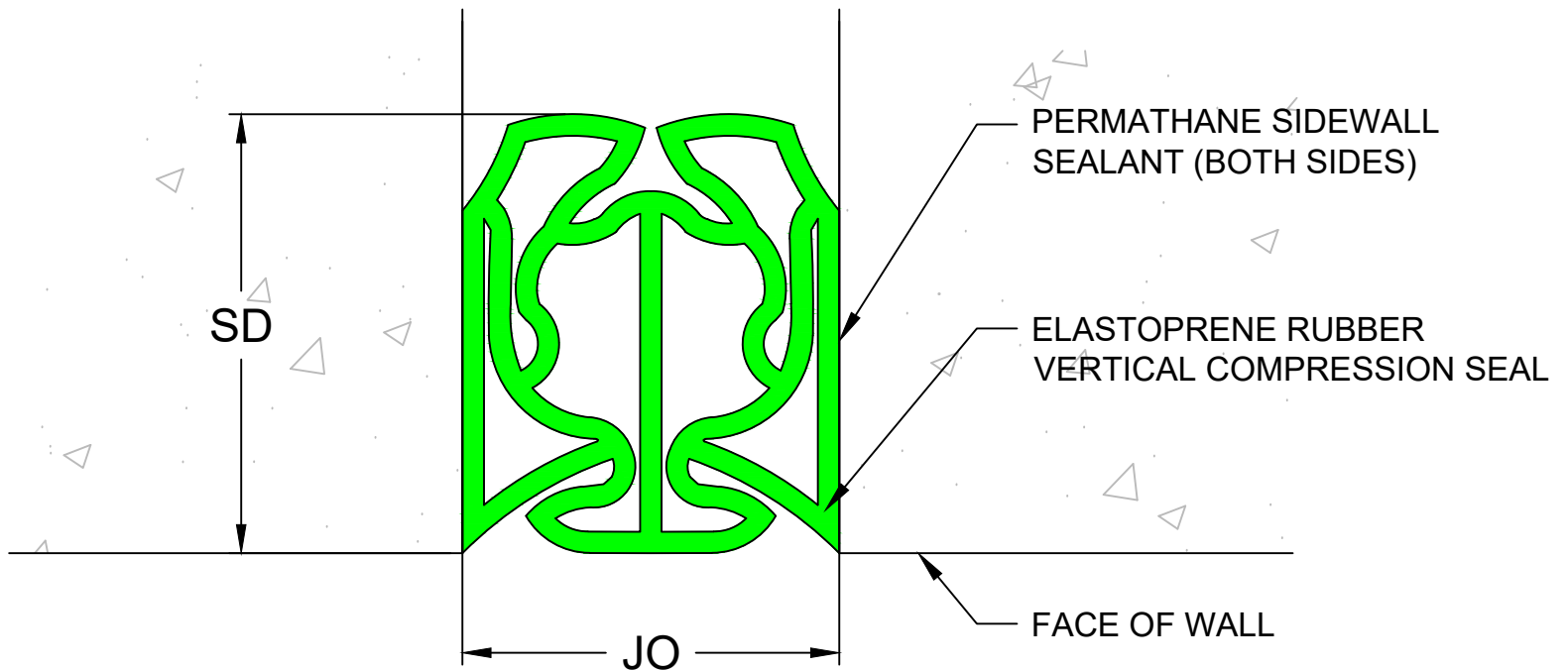
VCS Series Expansion Joint (Wall-to-Wall)
