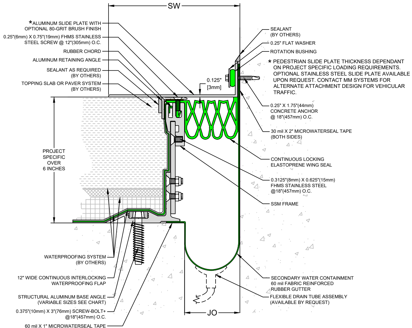
SSC-C Series Adjustable Height Expansion Joint Sizes 250 through 550 (Slab-to-Slab)
