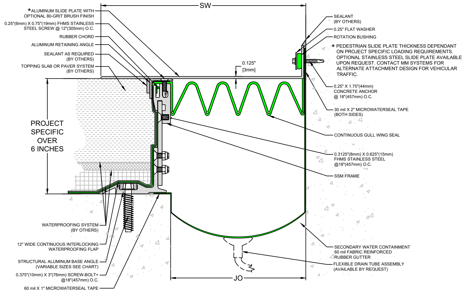
SSC-C Series Adjustable Height Expansion Joint Sizes 650 through 1200 (Slab-to-Slab)
