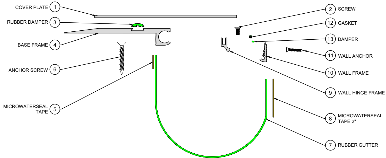
EXPLODED VIEW ▲
