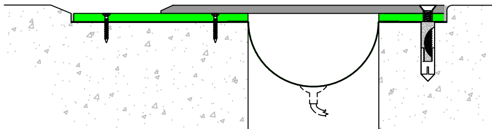
SID Series Expansion Joint Flat Cover (Slab-to-Slab)
