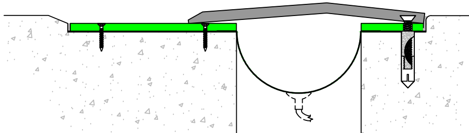
SID Series Expansion Joint Convex Cover (Slab-to-Slab)
