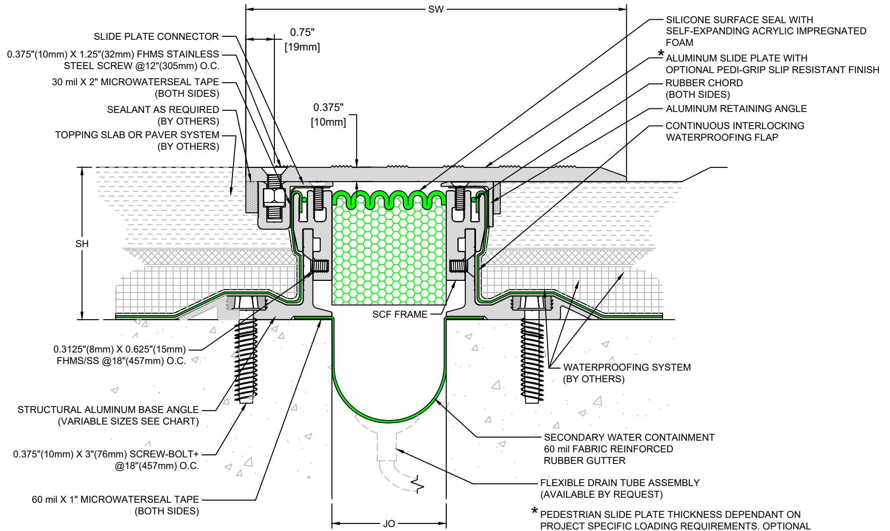
SCF Series Expansion Joint Sizes 150 through 600 (Slab-to-Slab)
