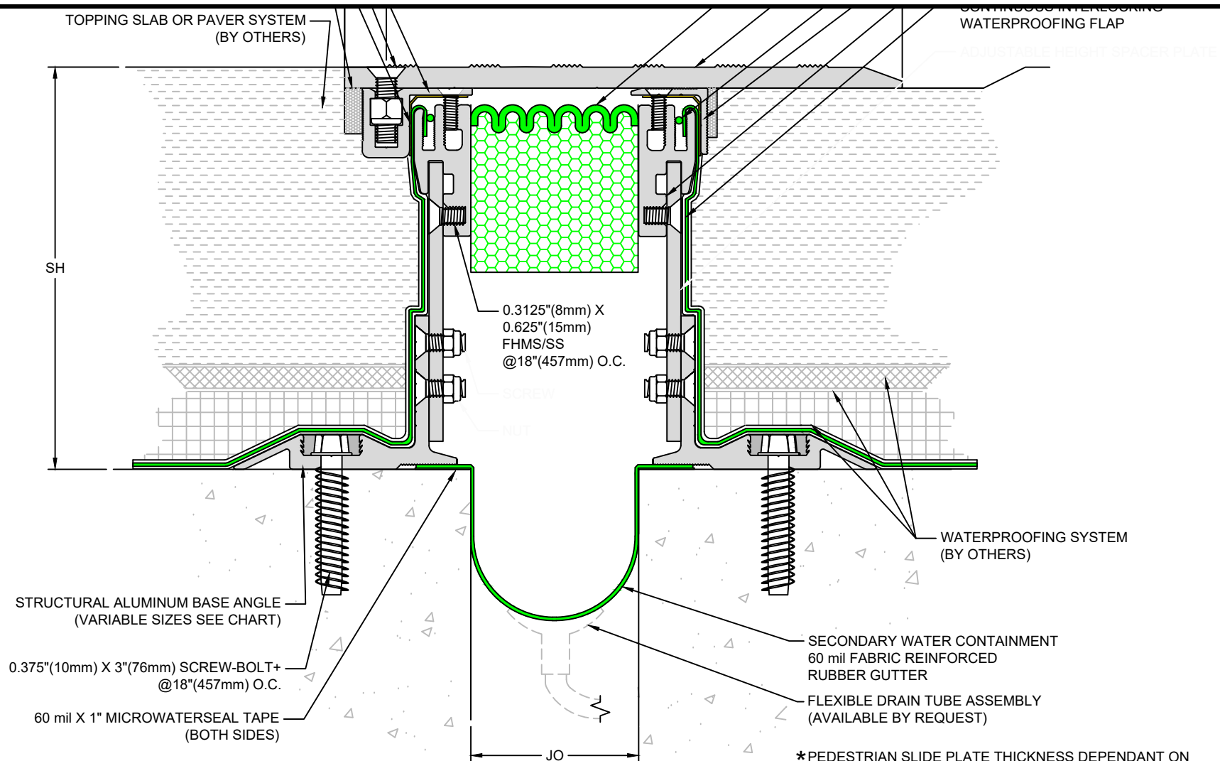
SCF Series Expansion Joint Sizes 150 through 600 (Slab-to-Wall)
