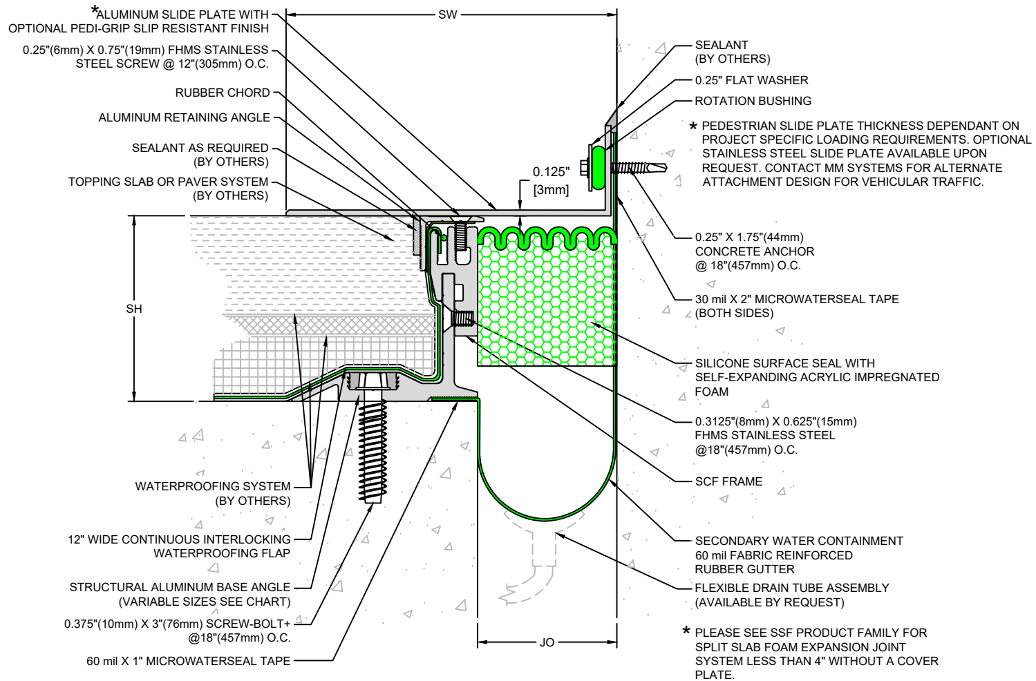
SCF-C Series Expansion Joint Sizes 150 through 600 (Slab-to-Wall)
