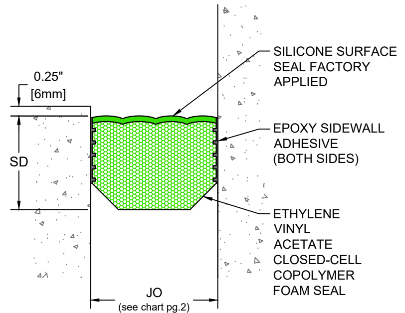
SCE-H Horizontal Series Expansion Joint Sizes 100 through 1200 (Slab-to-Wall)
