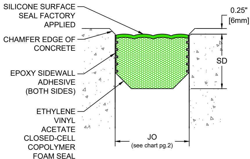
SCE-H Horizontal Series Expansion Joint Sizes 100 through 1200 (Slab-to-Slab)
