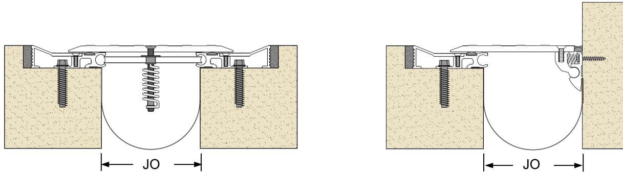
SSP Series (Slab-to-Slab)
