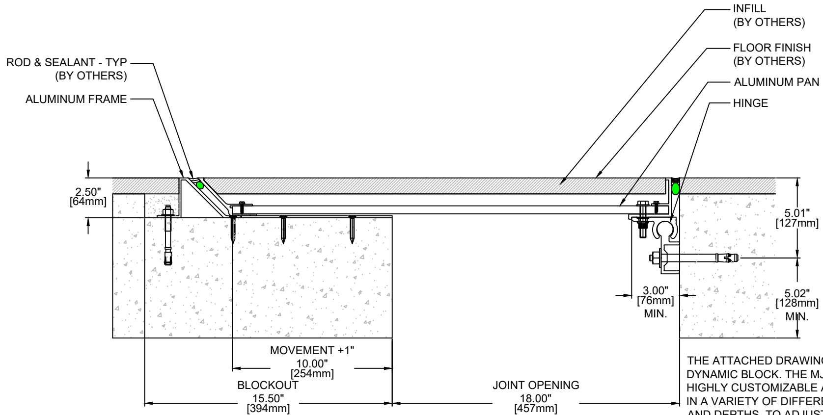
MJI Series Expansion Joint (Slab-to-Slab)
