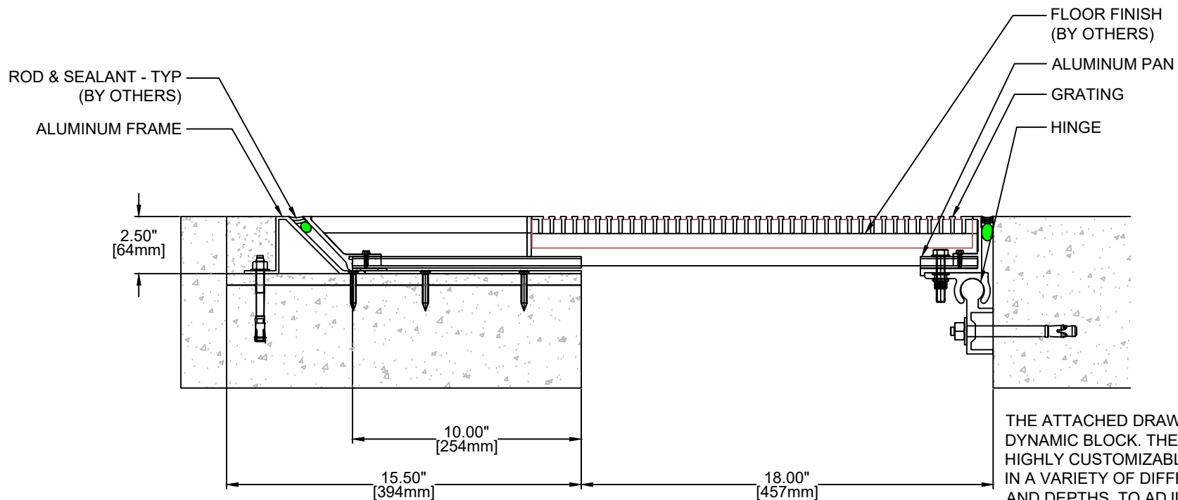
MJG Series Expansion Joint (Slab-to-Slab)
