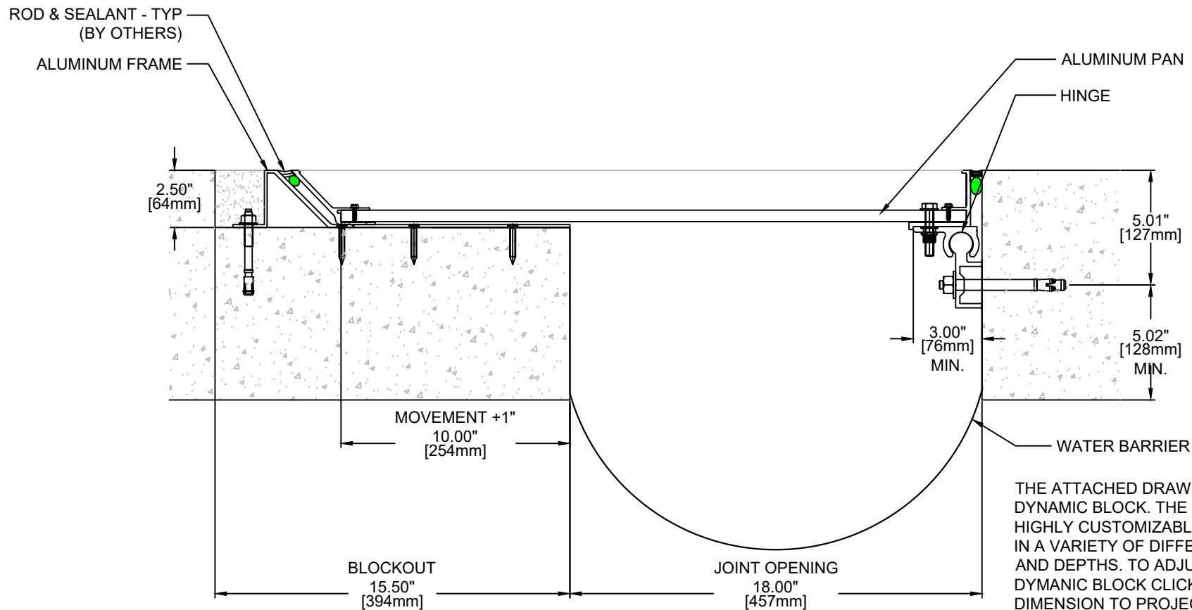
MJC Series Expansion Joint (Slab-to-Slab)
