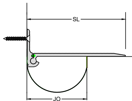
HFP-C (200-400) Expansion Joint (Slab to Wall)
