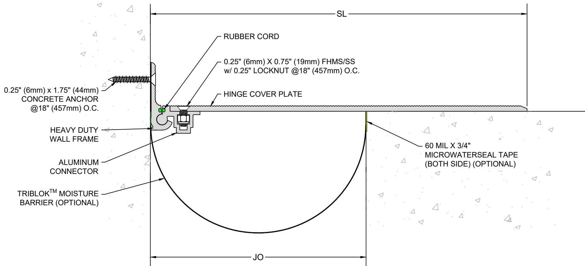
HFP-C Series Expansion Joint Sizes 600 through 1200 (Slab to Wall)
