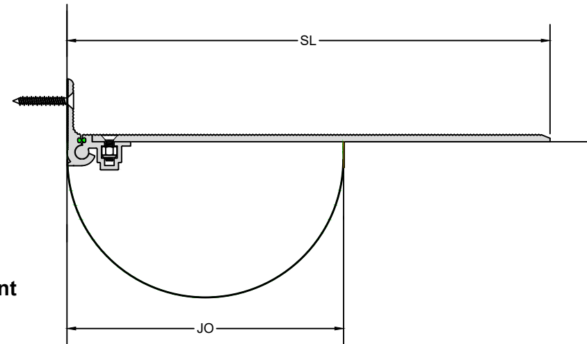
HFP-C (600-1200) Expansion Joint (Slab to Wall)
