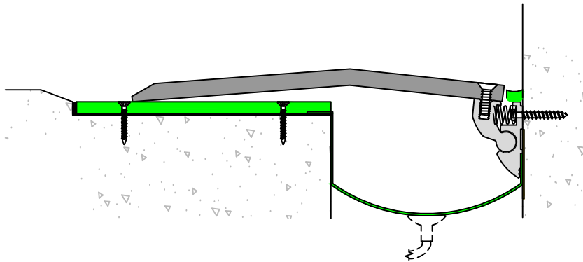
GID-C Series Expansion Joint Convex Cover (Slab-to-Wall)
