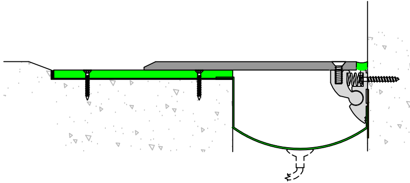
GID-C Series Expansion Joint Flat Cover (Slab-to-Wall)
