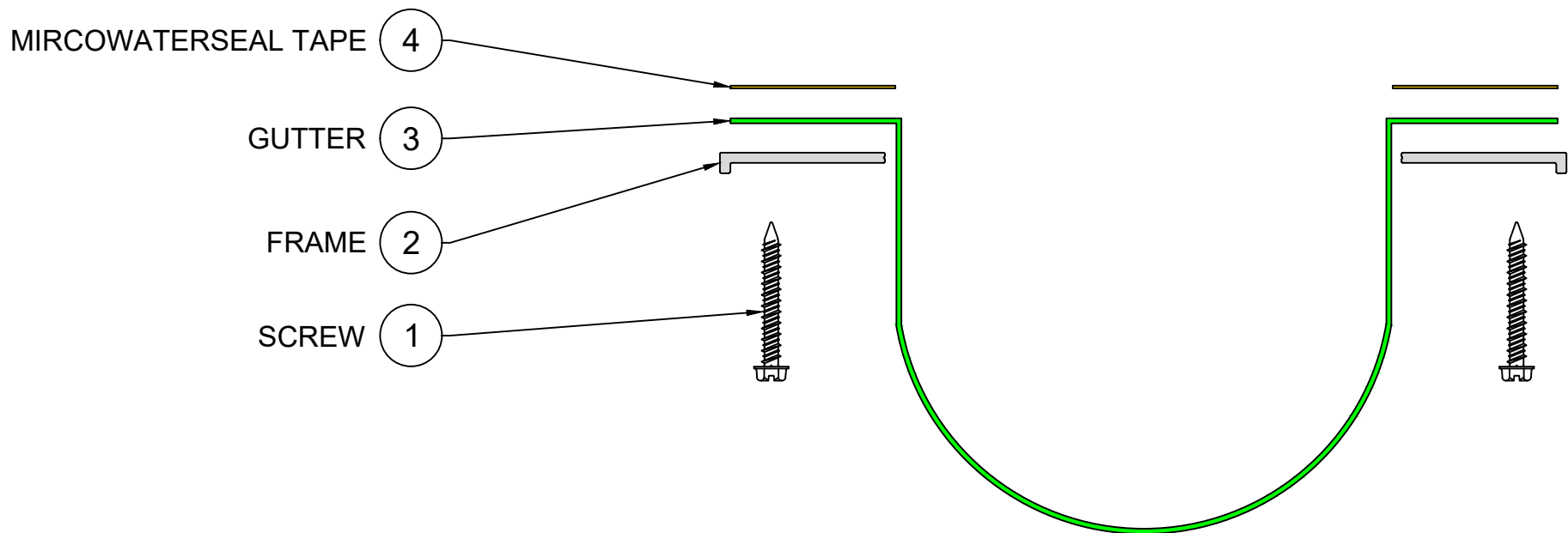
EXPLODED VIEW ▲ PART NUMBERS ▼
